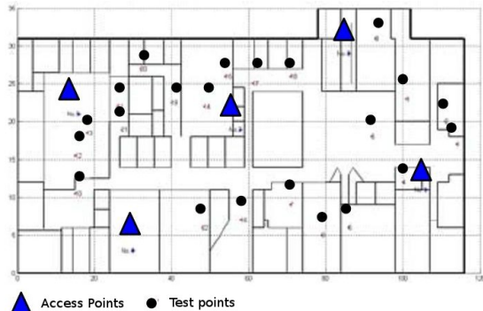
Fig. 2. UTBM test building and hardware and test points layout.
